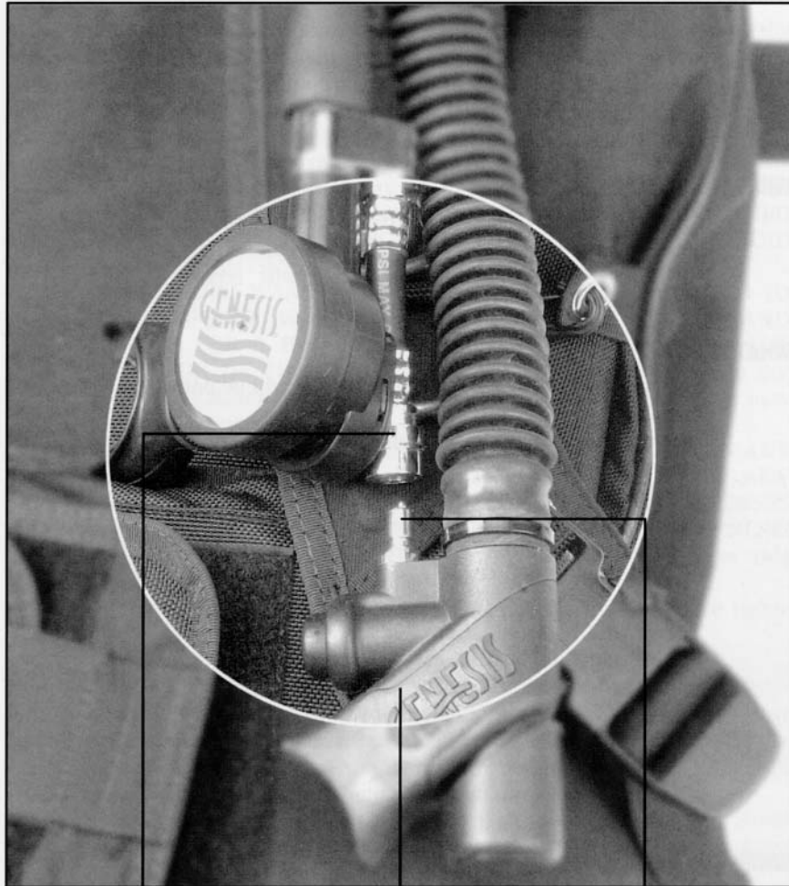
Quick-disconnect Coupler
